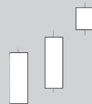
24) Deliberation (Bearish)
