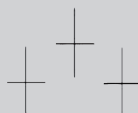
7) Kicking (Bearish)
